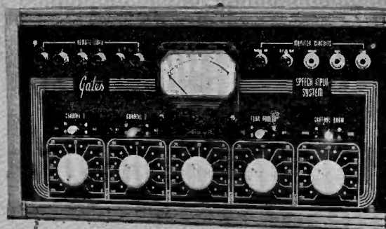
Model 51 CS Studioette Speech Input Console for smaller stations and sub-studio operation.
